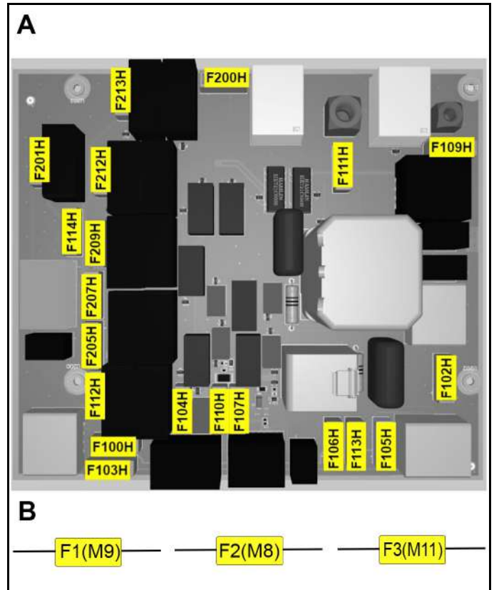
A: Fuses on the electronic controller
